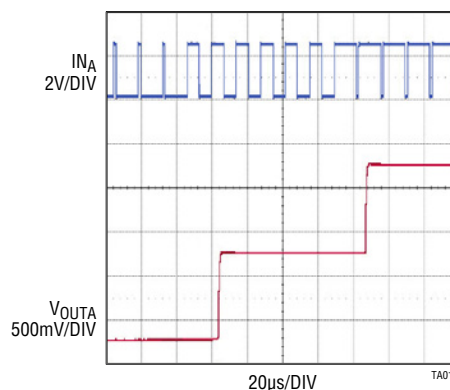
PWM Input to DAC Output
